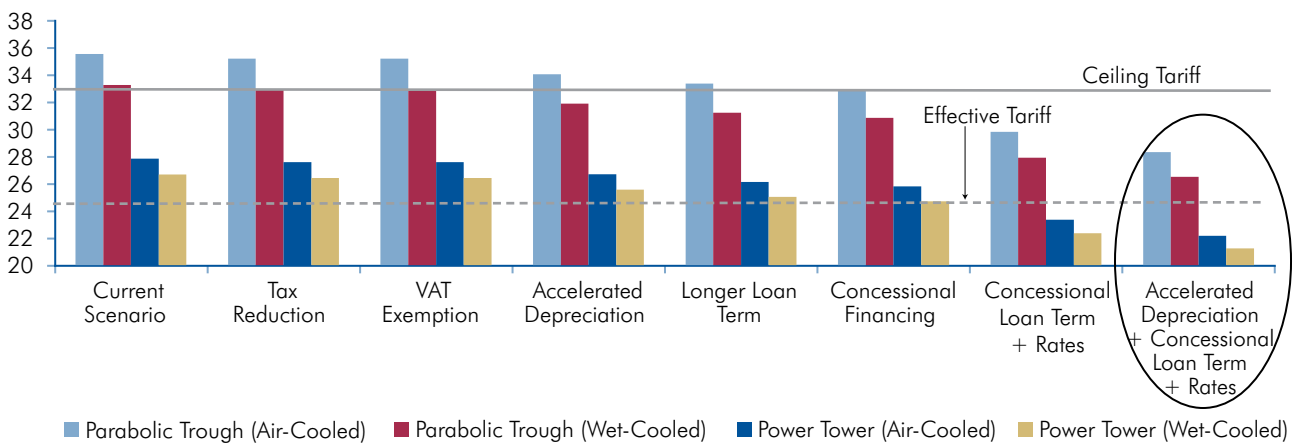
Figure 5.6: Impact Assessment of Different Regulatory Approaches on LCOE in India
