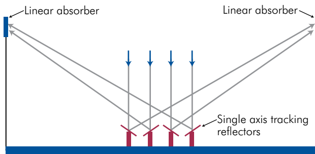
Figure A.6: Example of a CFLR System Source
