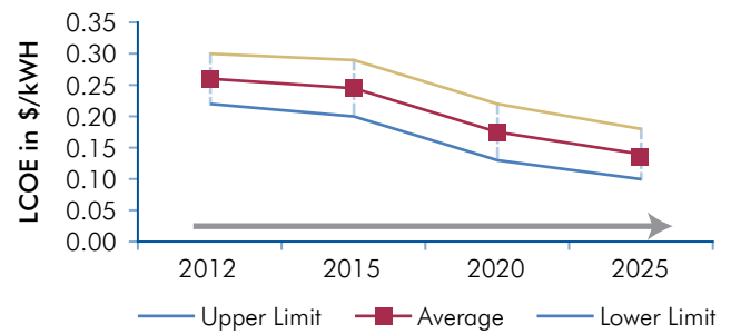
Figure 5.5: LCOE Reduction Potential for CST
