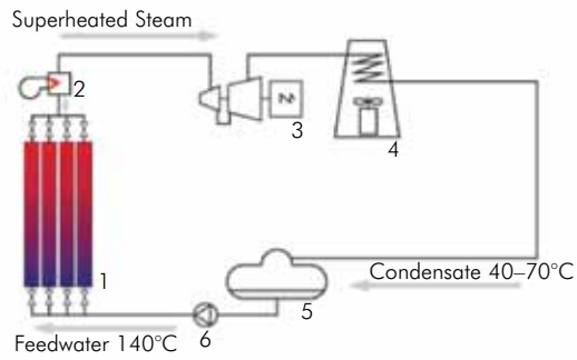
Figure A.12: Saturated Steam Hybrid Plant Configuration
