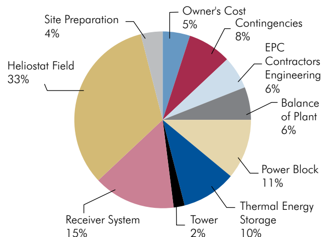
Figure 5.3: CAPEX Breakdown—Power Tower (100 MW – 15 h TES – US$978m)
