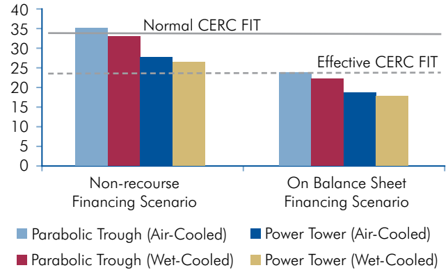
Figure 5.9: Balance Sheet vs. Off-Balance-Sheet Financing Effects on LCOE in India
