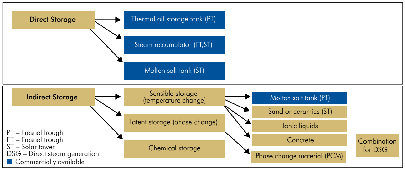
Figure A.11: Storage Concepts for CST
