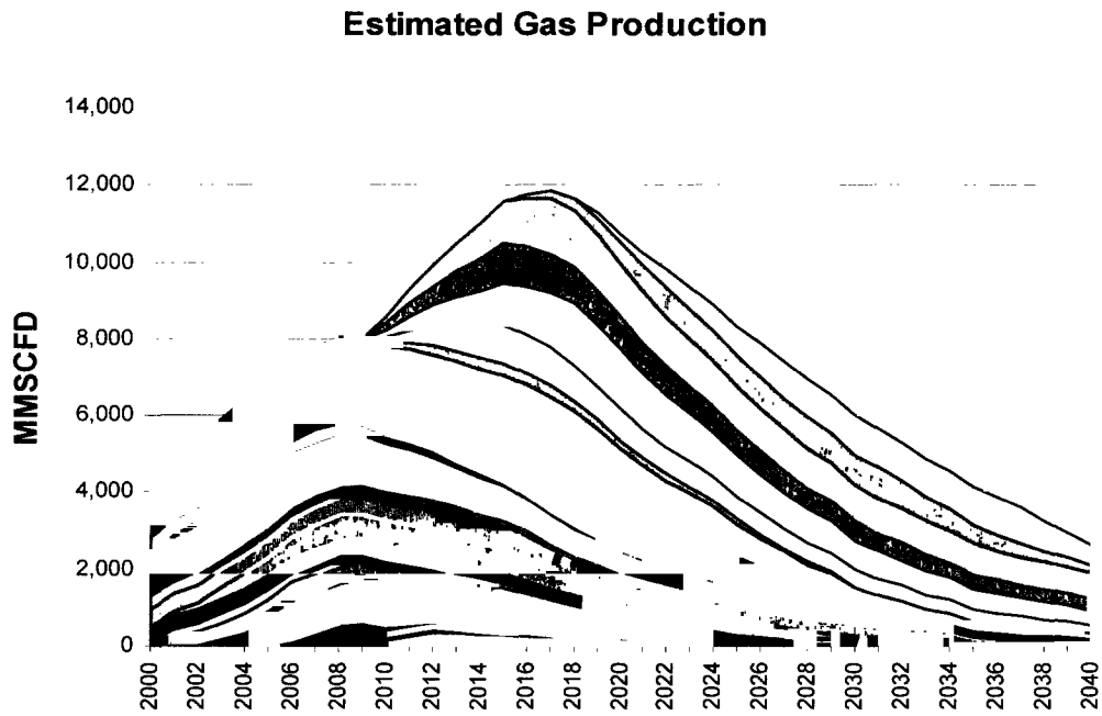
Figure 2.11: Gas Production Projections
