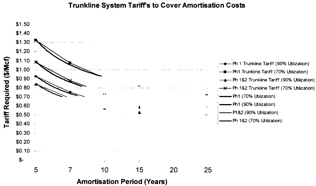
Figure 3.3: Countrywide Trunkline System Tariff Requirements
