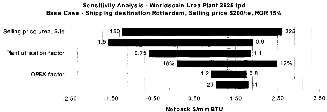
Figure A.2.12: Urea Sensitivity Analysis—Tornado Diagram
