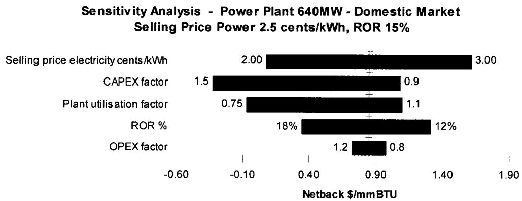
Figure A.2.19: Power Plant (domestic market) Sensitivity Analysis Tornado Diagram
