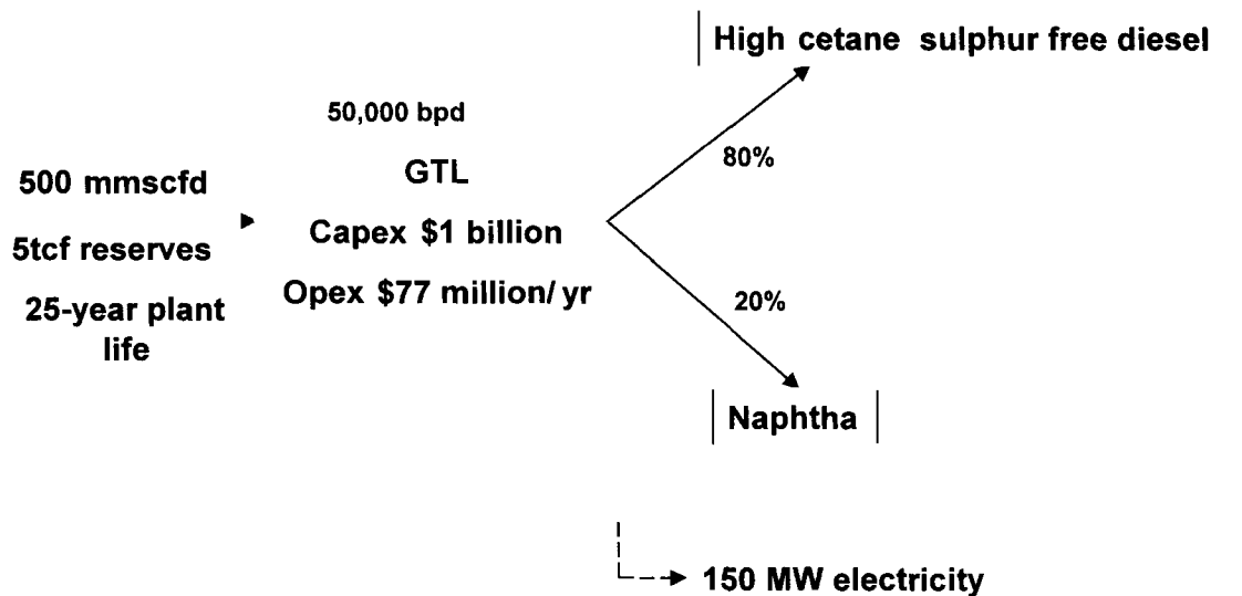
Figure A.2.6: GTL Typical Plant Economic Parameters
