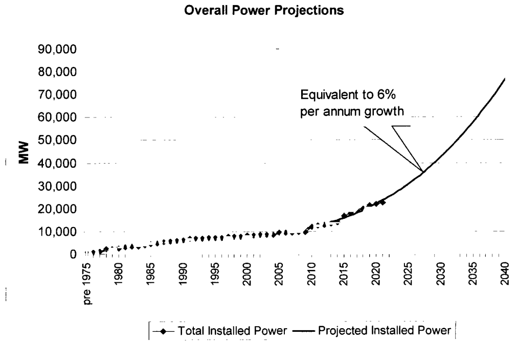
Figure 4.6: Power Demand Projection for Nigeria
