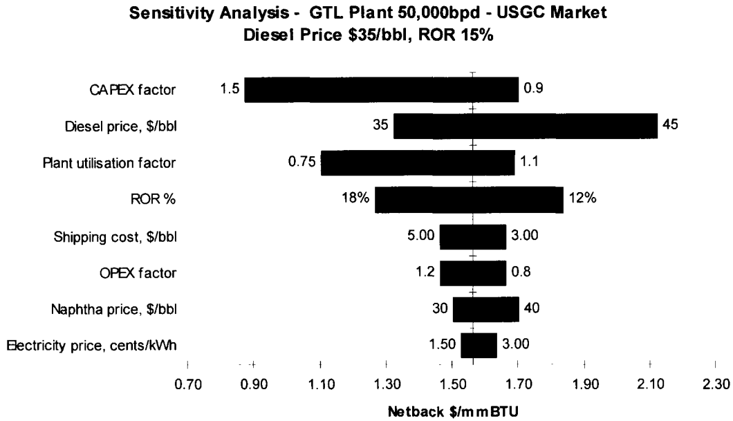
Figure A.2.17: GTL (50,000 Bpd) Sensitivity Analysis—Tornado Diagram
