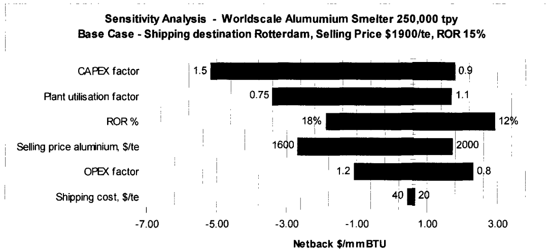
Figure A.2.14: Aluminum Sensitivity Analysis—Tornado Diagram
