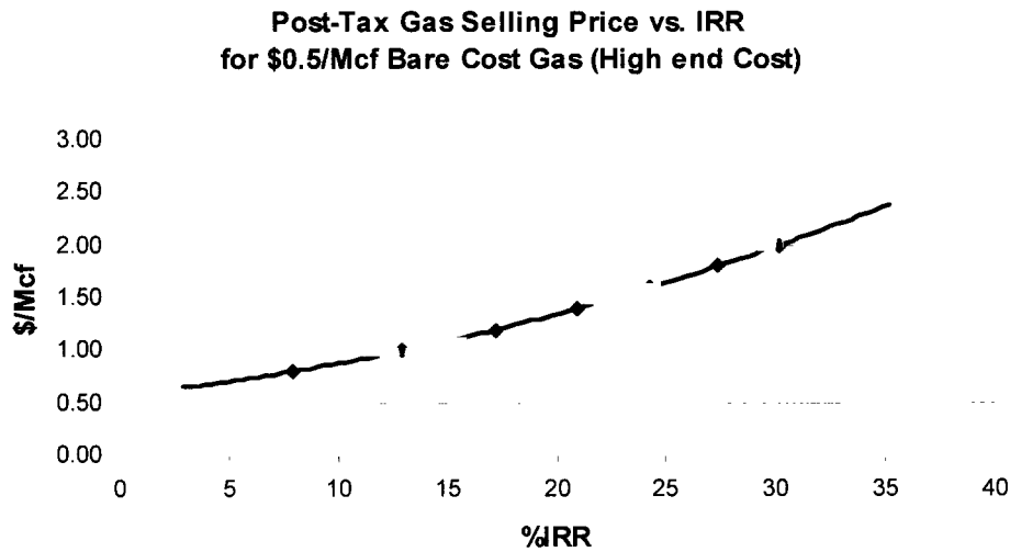
Figure 2.16: Post Tax Unit cost of Gas vs. IRR for US$0.50/mcf Gas (Based upon 15 percent Local and Foreign Company Overhead Cost)
