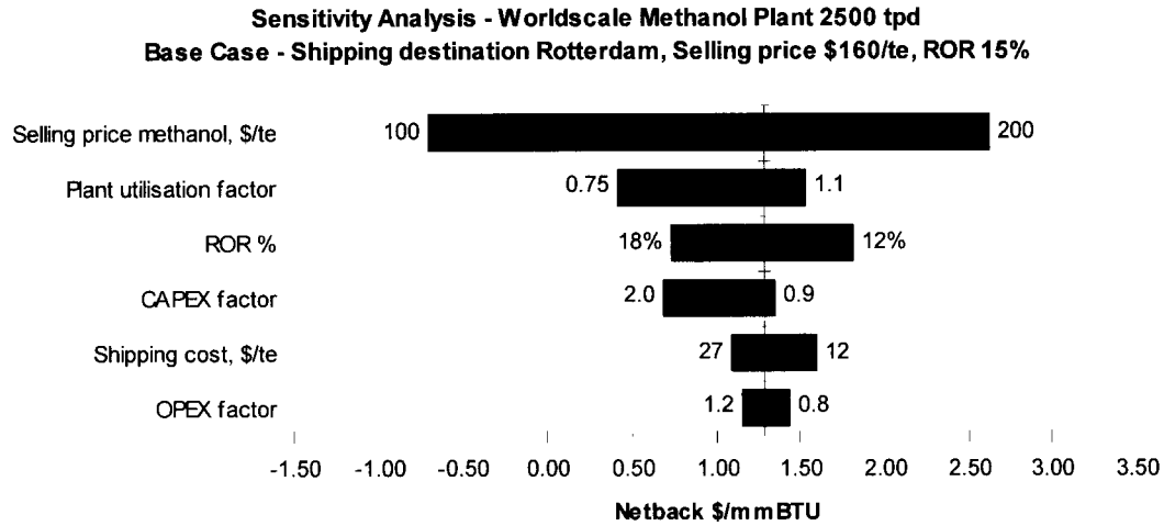
Figure A.2.10: Sensitivity Analysis Diagram
