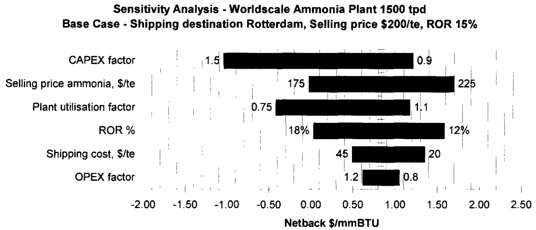
Figure A.2.11: Ammonia Sensitivity Analysis—Tornado Diagram
