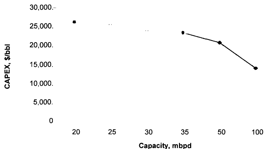
Figure A.2.7: GTL Plant Capital Investment
