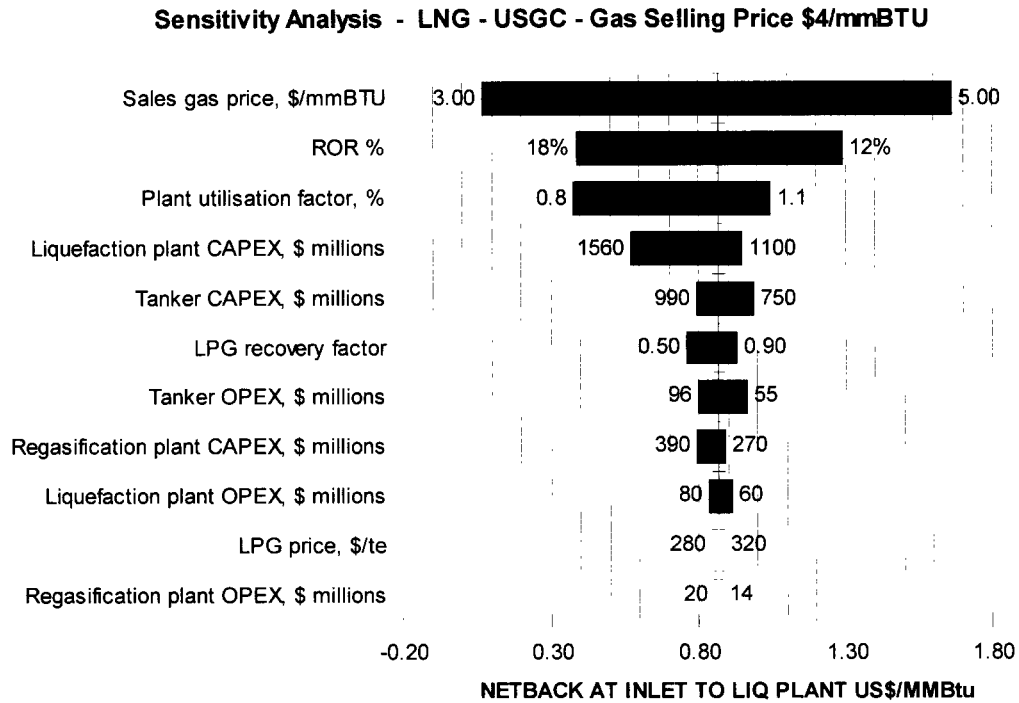
Figure A.2.18: LNG Sensivity Analysis—Tornado Diagram
