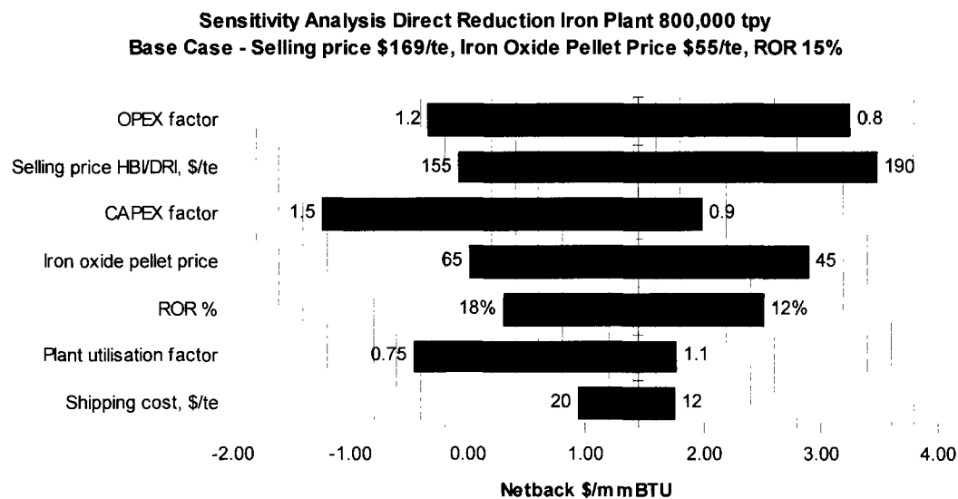
Figure A.2.15: Steel (DRI) Sensitivity Analysis—Tornado Diagram
