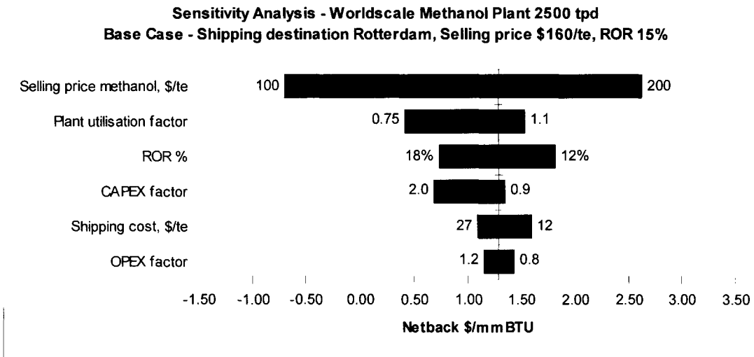
Figure A.2.13: Methanol Sensitivity Analysis—Tornado Diagram
